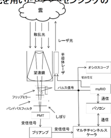
図1 lidar system (monostatic)
